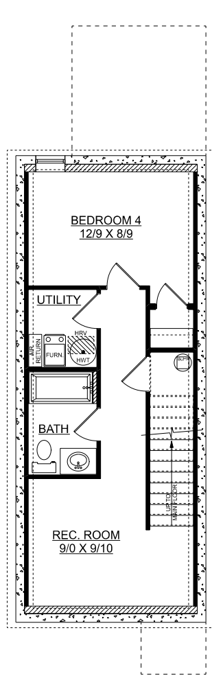
OPTIONAL BASEMENT PLAN 431 SQ. FT.
