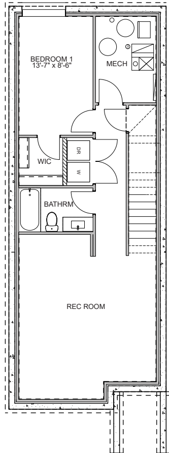
OPTIONAL BASEMENT PLAN 579 SQ. FT.
