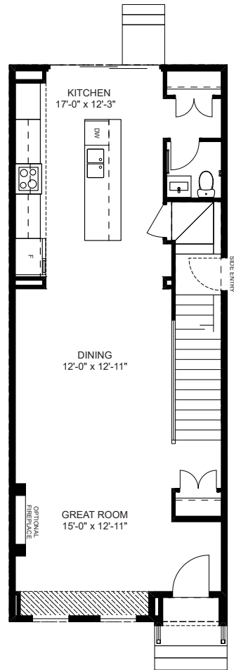
MAIN FLOOR PLAN 816 SQ. FT.
