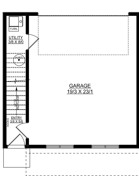
MAIN FLOOR PLAN 75 SQ. FT.
