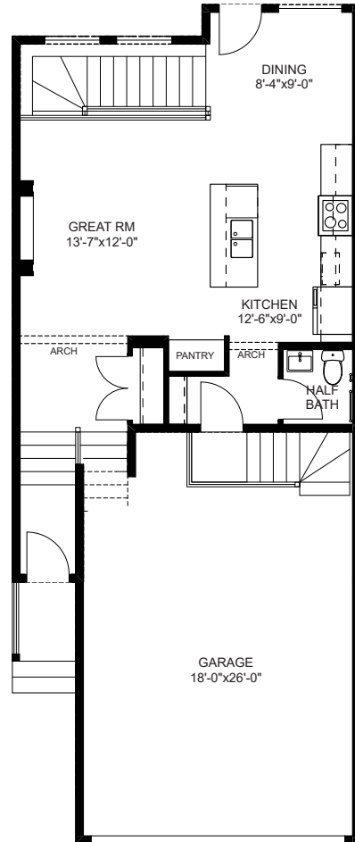
MAIN FLOOR PLAN 632 SQ. FT.
