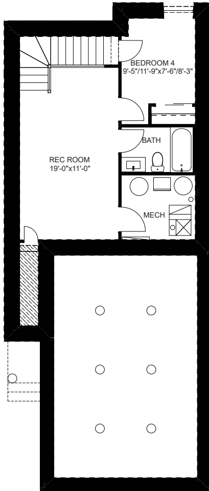
OPTIONAL BASEMENT PLAN 383 SQ. FT.
