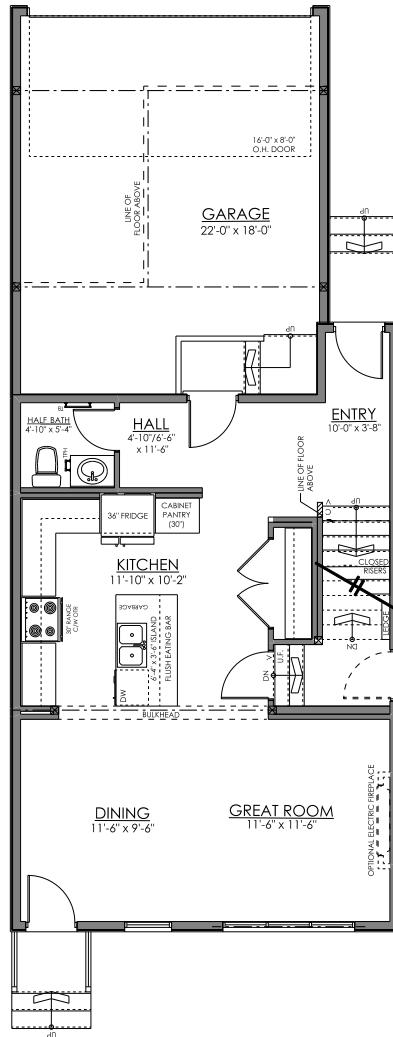
MAIN FLOOR PLAN 690 SQ. FT.
