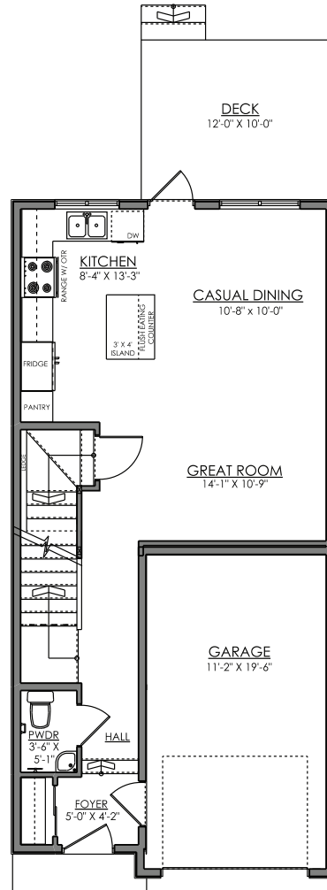
MAIN FLOOR PLAN 594 SQ. FT.
