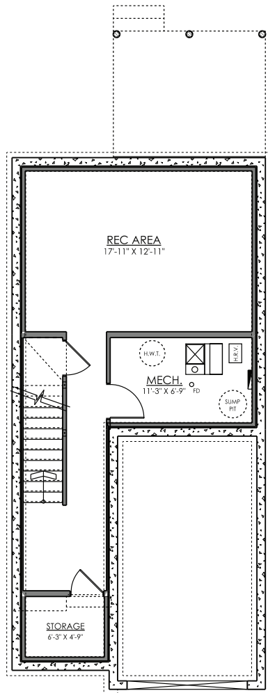
OPTIONAL BASEMENT PLAN 373 SQ. FT.
