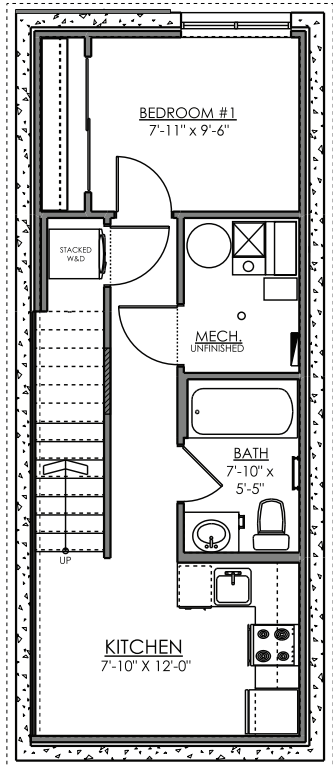
OPTIONAL BASEMENT SUITE 329 SQ. FT.
