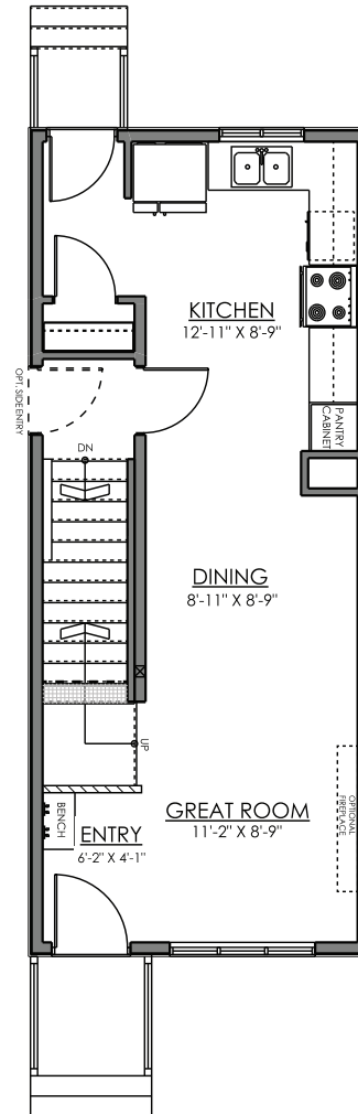
MAIN FLOOR PLAN 476 SQ. FT.
