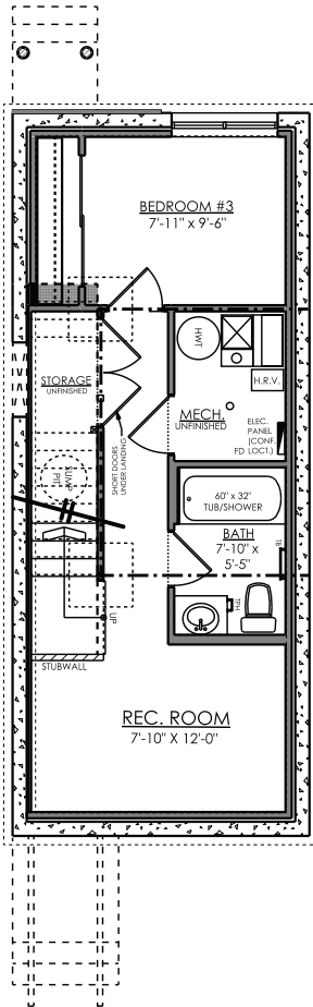
OPTIONAL BASEMENT PLAN 325 SQ. FT.
