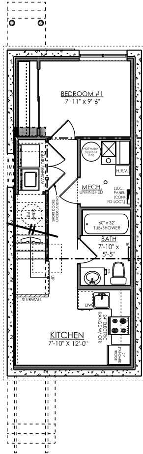
OPTIONAL BASEMENT SUITE 342 SQ. FT.
